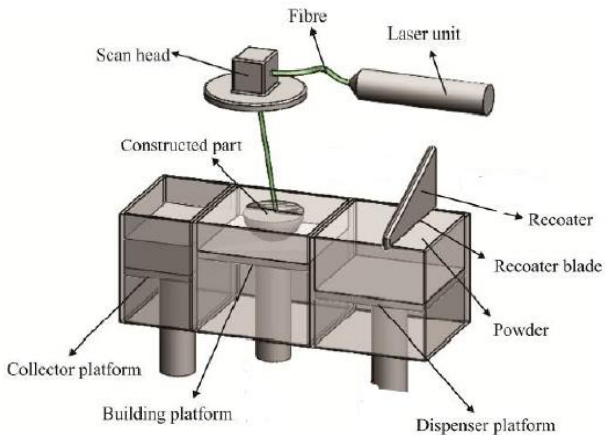
Figure 2.7: Schematic diagram of a DMLS system [33]
