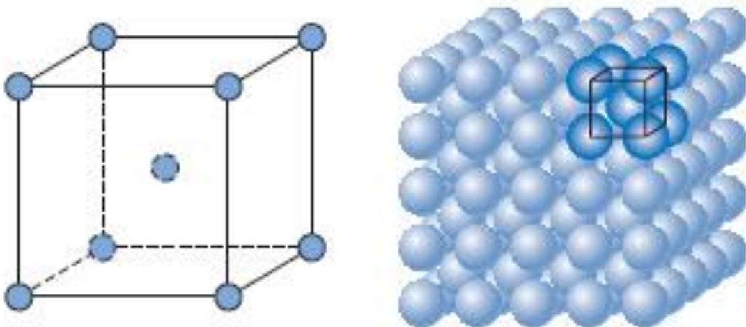
Figure 2.2: The body-centred cubic crystal structure. Left: a reduced-sphere unit cell, and right: an aggregate of many atoms [23]
