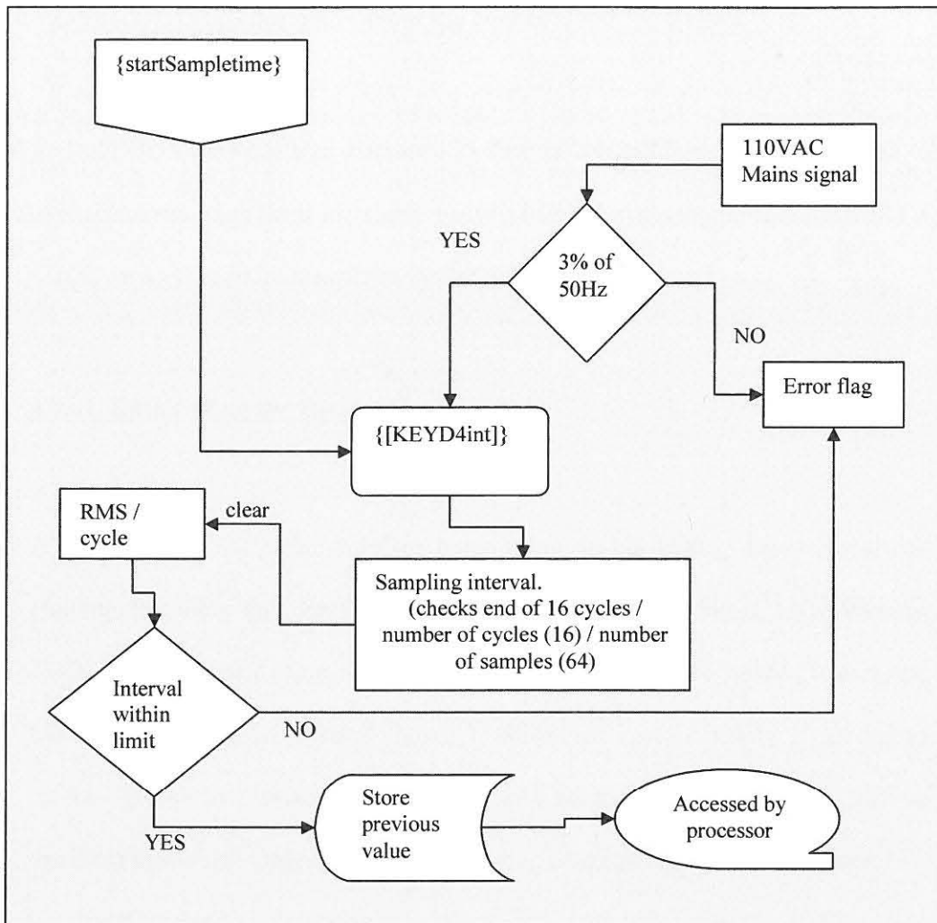
Fig. 4.14. Flow diagram of the microcontroller hardware interrupt environment to start cycle measurement on the CME12-A4 single phase prototype.
