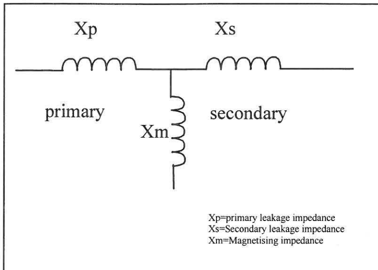
Fig. 2.5. T-equivalent model of a transformer [10, p. 7].
