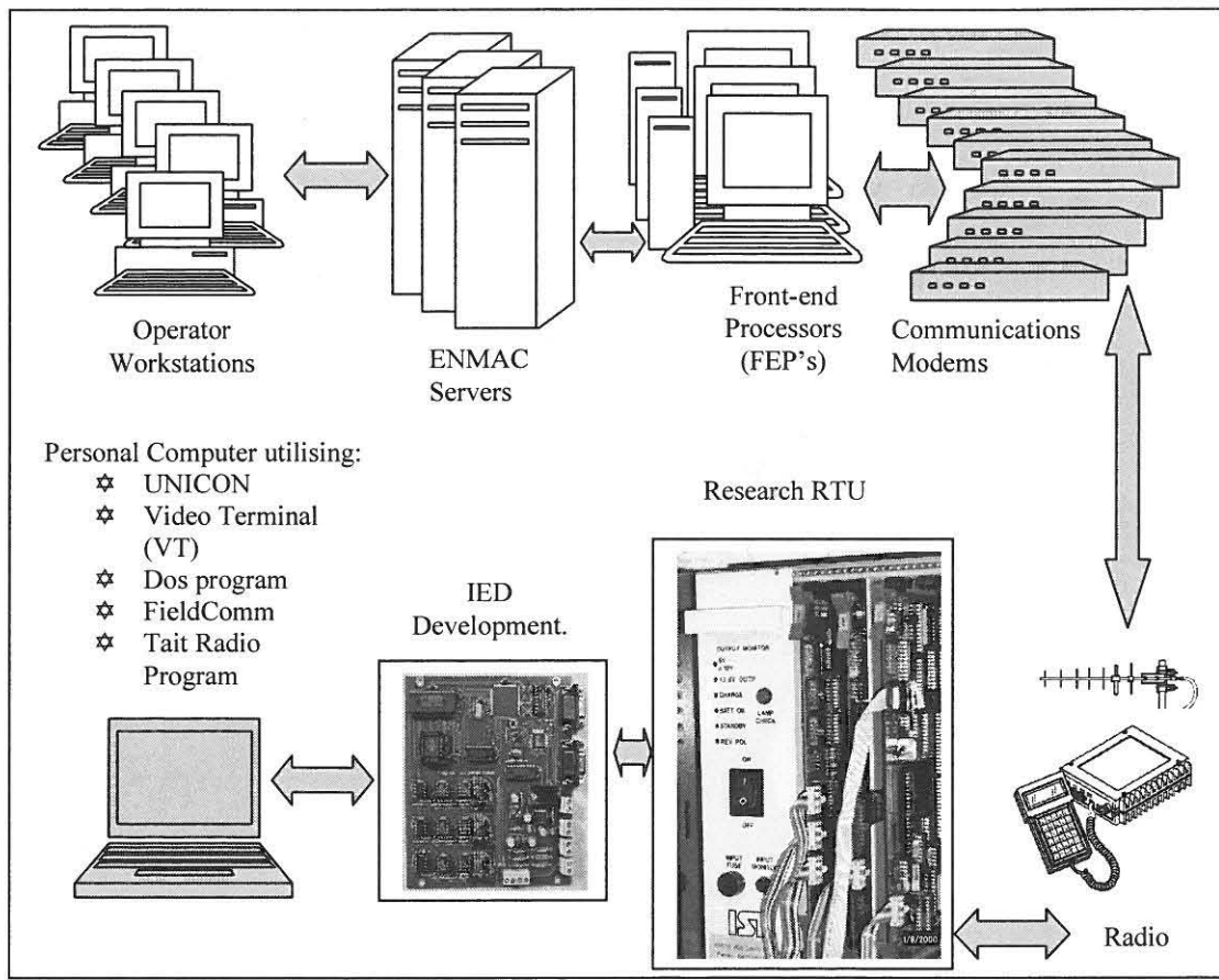
Fig. 4.20. Final hardware configuration setup as used for the evaluation period.
