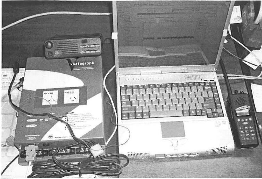
Fig. 6.5. The Vectograph that was used for test comparison and as a reference of the readings during this research.
