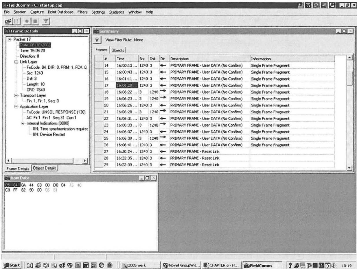
Fig. 6.6. Application layer message from RTU to Master requesting time synch.
