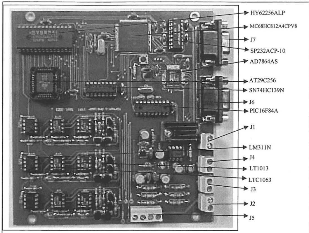
Fig. 4.6. The final IED quality of supply measuring device, using the MC68HC812A4CPV8 microcontroller.
