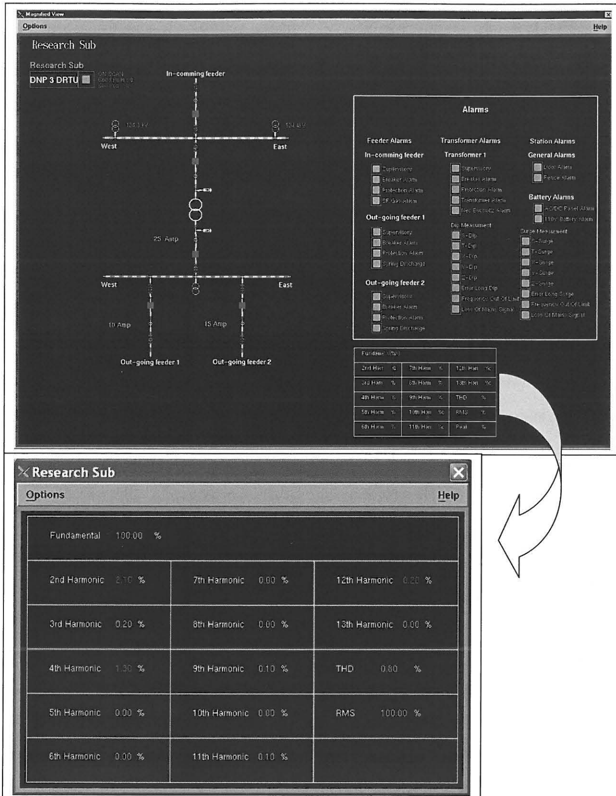
Fig. 6.35. The final layout of the substation on the ENMAC, showing harmonic and voltage dip states.
