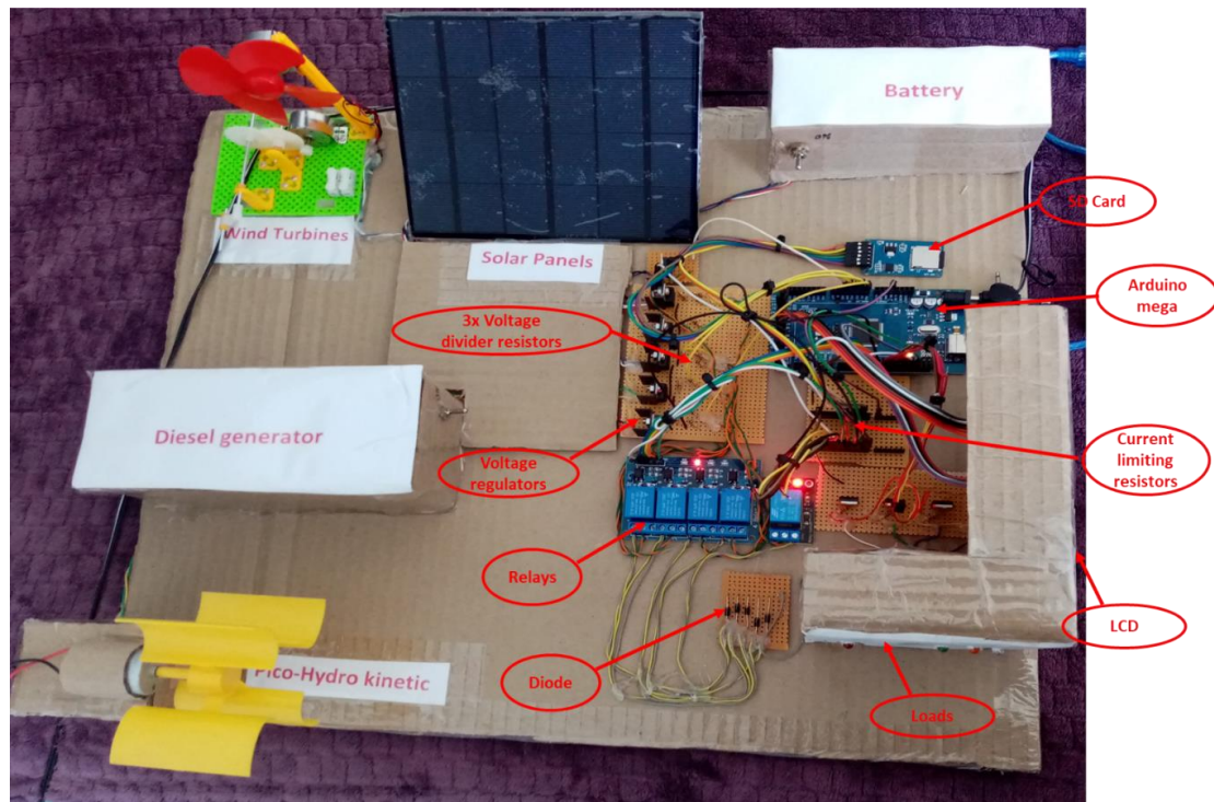
Figure 5.6: Practical Setup
