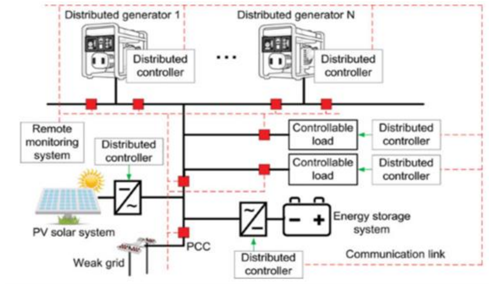
Figure 2.8: Microgrid with distributed control structure [111]
