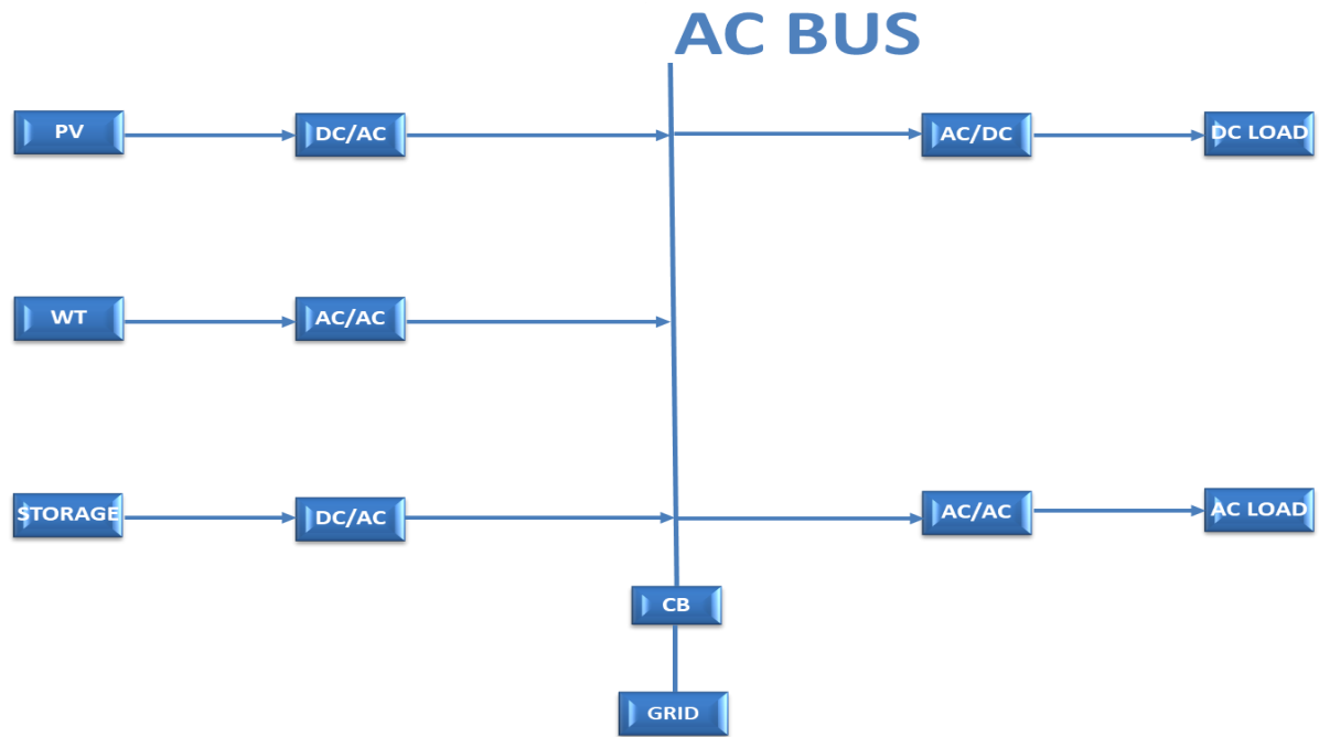
Figure 2.3: AC microgrid block diagram
