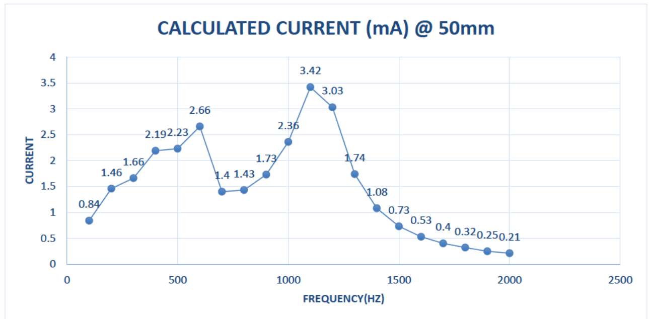
Figure 4.27 Calculated current with coils at 50 mm and load of 10 k \Omega
