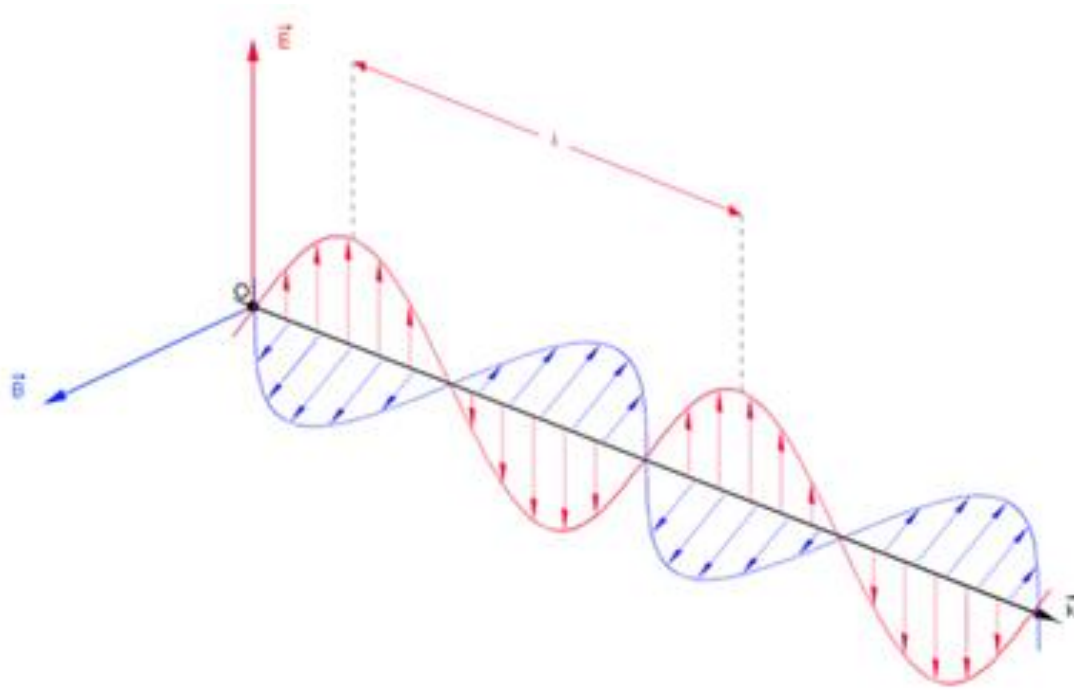
Figure 2.8 Electromagnetic waves
