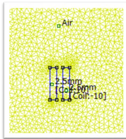
Figure 4.2 A single-layer helix coil drawn in FEMM software
