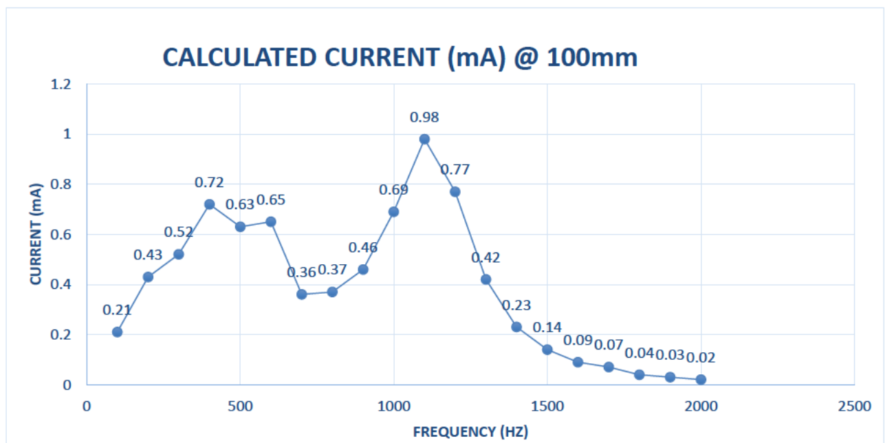
Figure 4.25 Calculated current with coils at 100mm and load of 10 k \Omega
