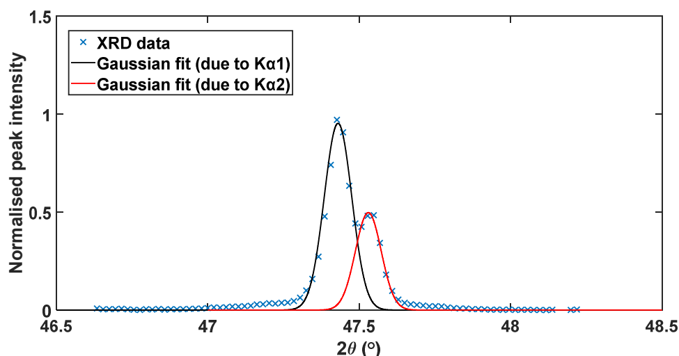
Figure 9. A typical measured XRD data, with the K\alpha_1 and K\alpha_2 deconvoluted peaks using a Gaussian function of (1011) reflection.
