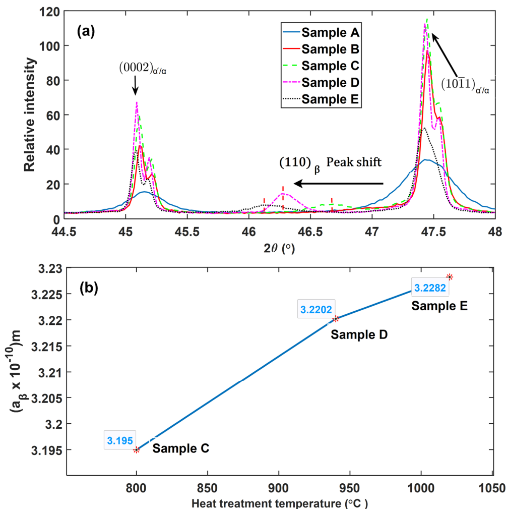
Figure 7. (a) The magnification of selected peaks (110)_{\beta} , (0002)_{\alpha/\alpha} and (10\bar{1}1)_{\alpha/\alpha} , (b) Evolution of the \beta -phase lattice parameter \{a\} with heat treatment temperatures.
